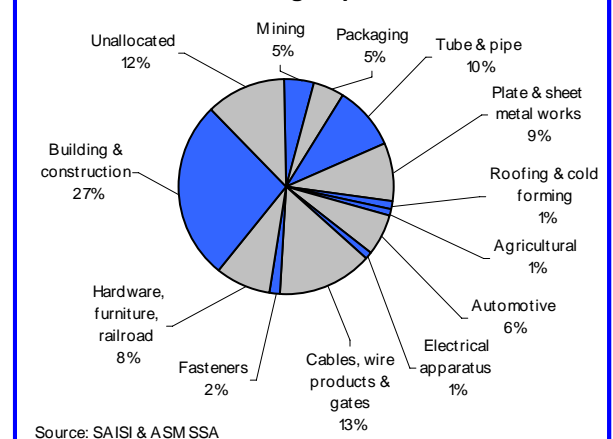
Sales of primary carbon steel products to industrial groups - Q3 2007
