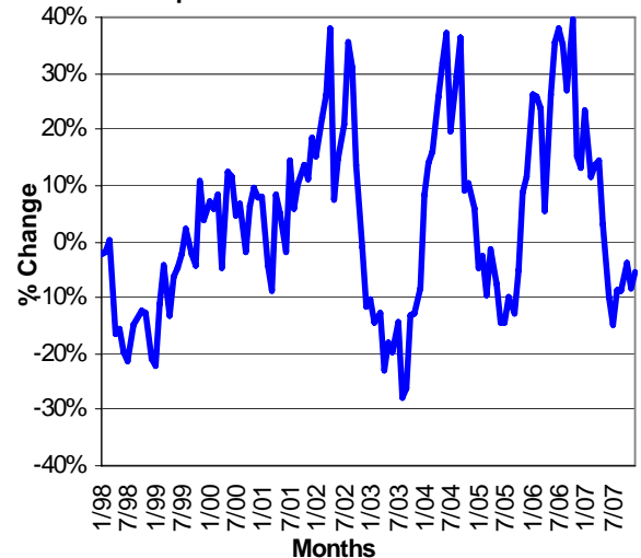
Change* in local sales of primary carbon steel products Jan 1998 - Dec 2007
